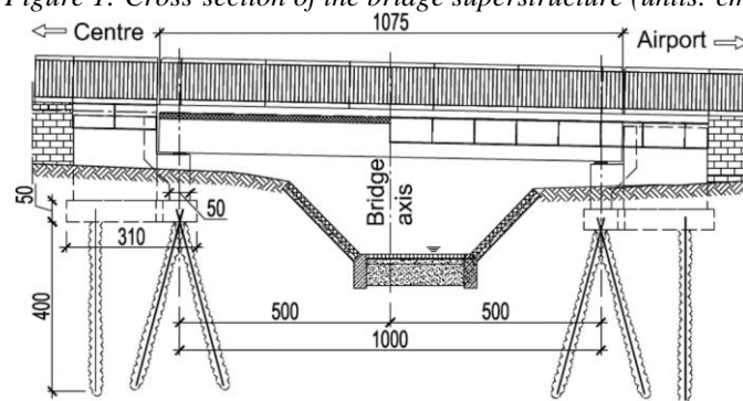
Figure 2: Side view and longitudinal section of the bridge (units: cm)
