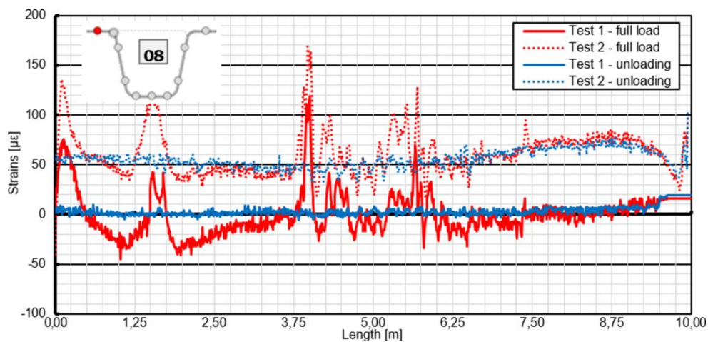
Figure 8: Graph of the strains measured with the DFOS no. 08 - the upper flange of G2
