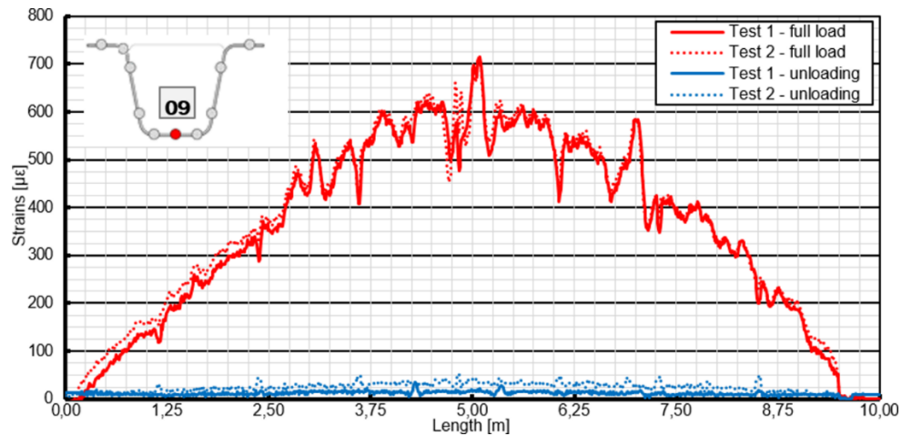
Figure 7: Graph of the strains measured with the DFOS no. 09 - the bottom flange of G1
