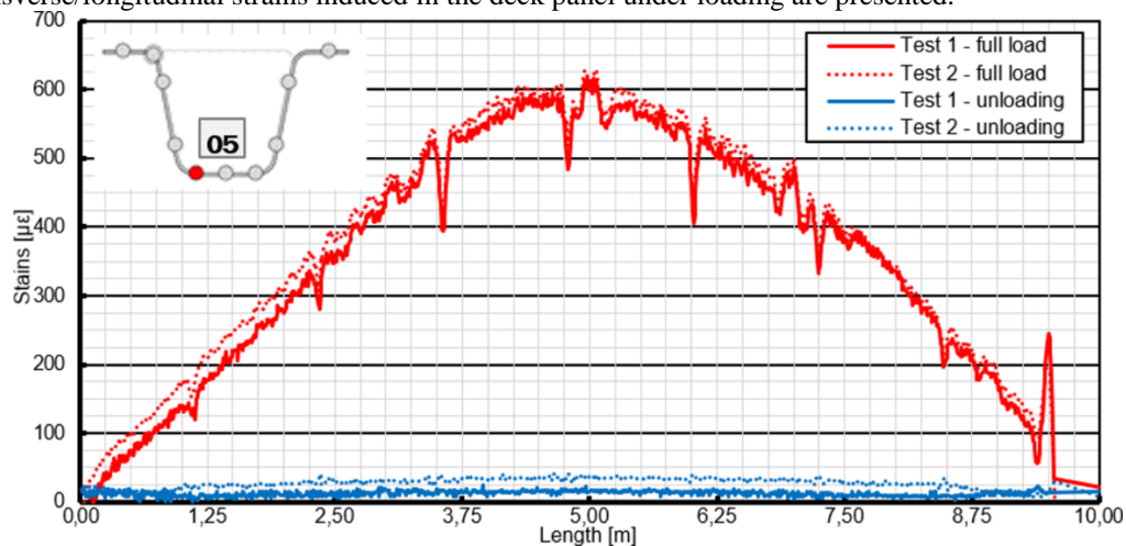
Figure 6: Graph of the strains measured with the DFOS no. 05 – the bottom flange of G1
