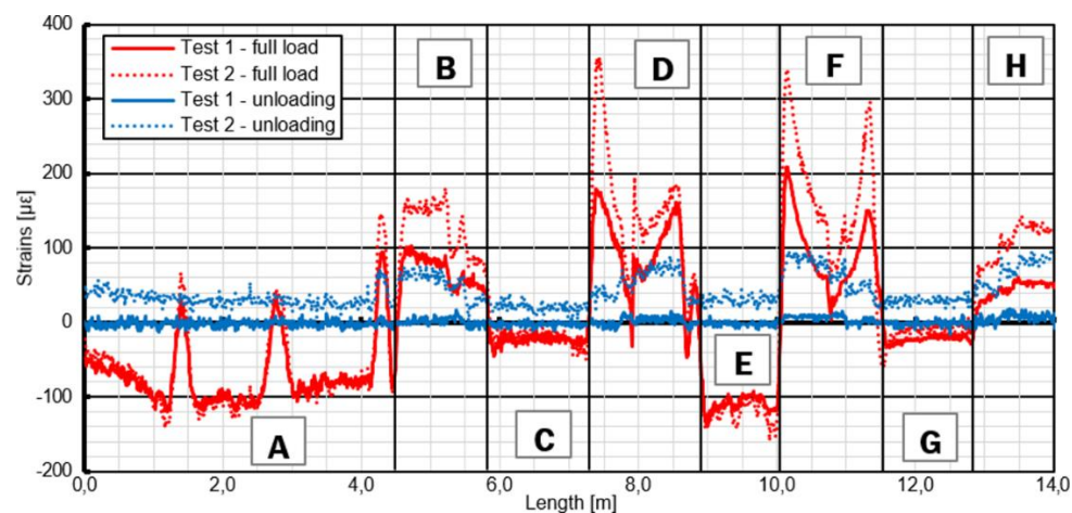
Figure 9: Graph of the strains measured with the DFOS no. 03 - the bottom surface of the deck panel
