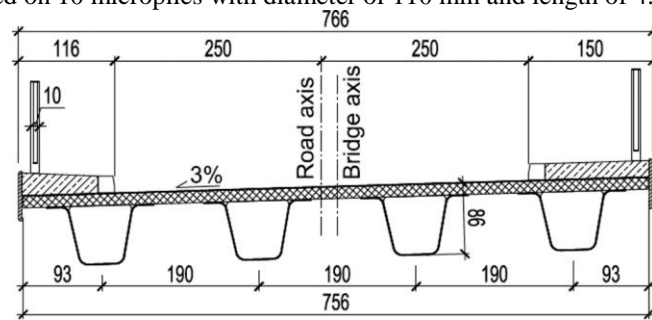
Figure 1: Cross-section of the bridge superstructure (units: cm)
