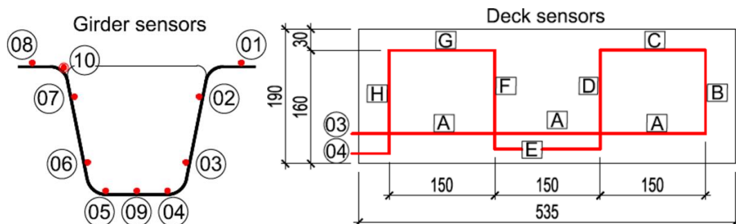
Figure 3: Sensor layout for the girder and deck panel strains measurement (sensor no. 10 for temperature only)
